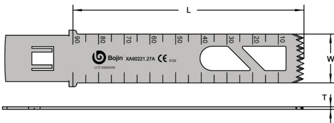
Saw blade(Aesculap)
