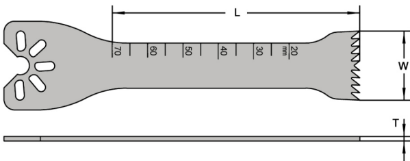
Saw blade(Microair)
