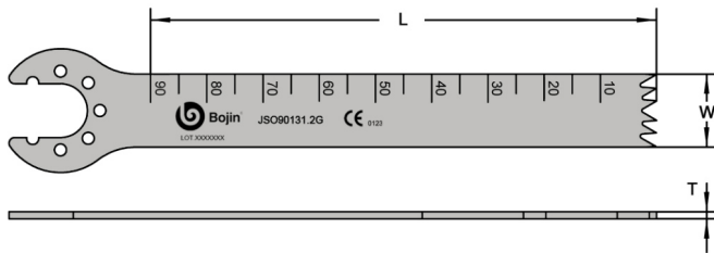
Saw blade(Microair)
