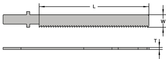
Reciprocating saw blade
