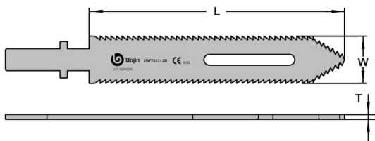
Reciprocating saw blade
