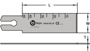
Saw blade(Bojin system 8000)
