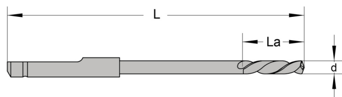
Cutting drill bit
