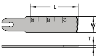
Saw blade(Bojin system 3000)
